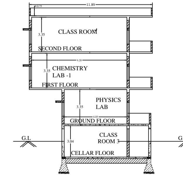
SECTION
